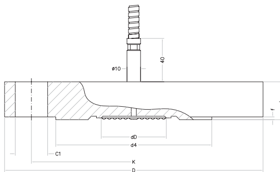
Capillary execution
