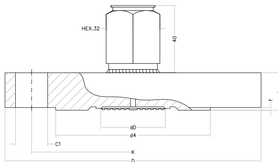
Threaded execution
